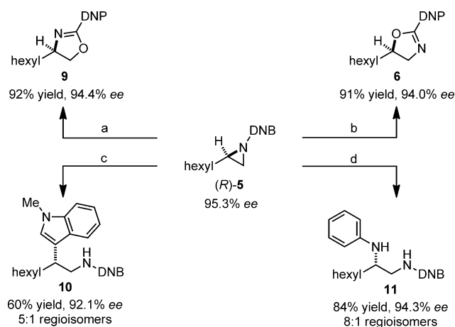
Scheme 4. Ring opening reactions of enantioenriched 5 . a) NaI (10 mol %), THF, 60 °C, 12 h. b) TfOH (10 mol %), DCM, 0–25 °C, 2 h. c) Zn(OTf) 2 (20 mol %), N -methylindole (4 equiv), DCM, 25 °C, 18 h. d) Zn(OTf) 2 (20 mol %), aniline (4 equiv), DCM, 25 °C, 18 h.
